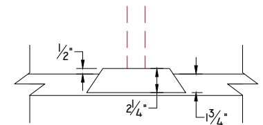
SIDE POCKET PLAN VIEW SCALE: 1" = 1'-0"
